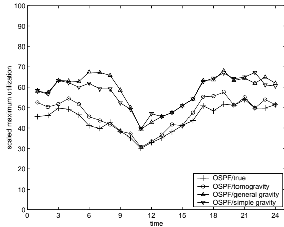
(b) The '+' signs show the performance of the OSPF optimization using the true traffic matrix, and the circles, \Delta and \nabla show the OSPF optimization on the tomogravity, general and simple gravity model estimates, respectively.
