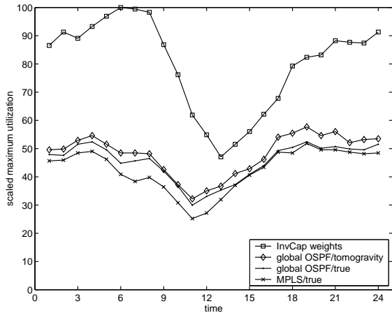
Figure 5: Global optimization over a 24 hour period. Once again the crosses represent the optimal solution for each one hour data set, and the squares represent inverse capacity weights. The points, and diamonds represent the global optimum weights calculated from the set of real and estimated traffic matrices, respectively, applied to each one hour traffic matrix.
