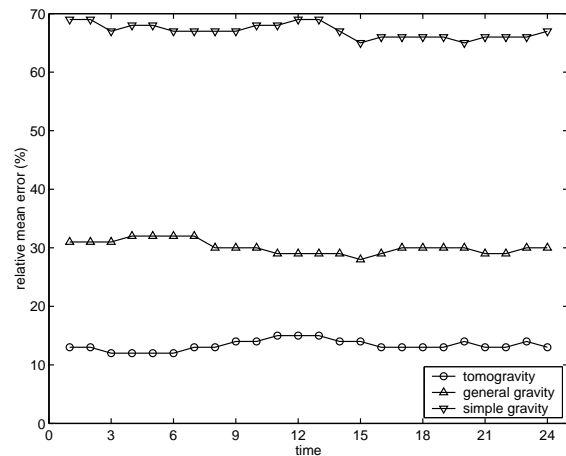
Figure 2: Relative error for the different traffic estimates for each of the 24 hours. The circles show the tomogravity estimate, and the \triangle and \nabla show the general and simple gravity model estimates. For tomogravity, the average relative error is 0.13, for general gravity it is 0.30, and for simple gravity it is 0.67.
